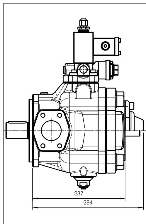
01 PHPK 3-(80-100-120) + Option "A" Single stage of pressure
