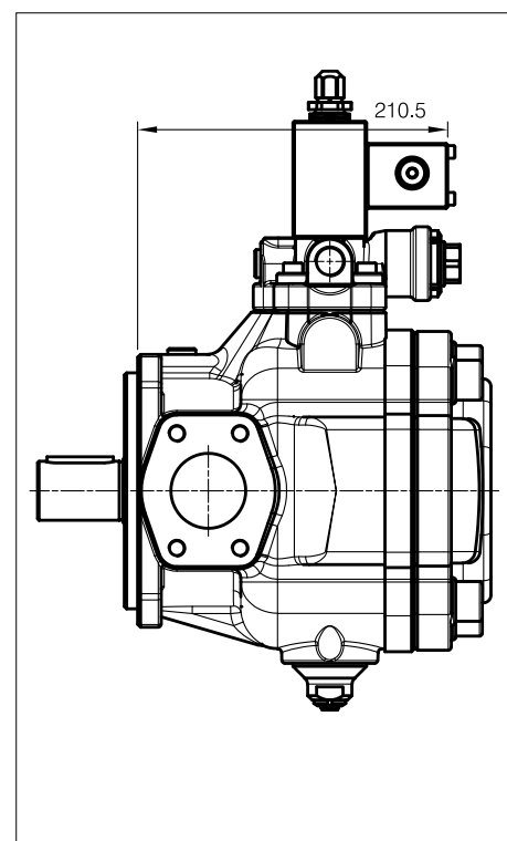
01 PHPK 3-(80-100-120) PCS003 pressure control
