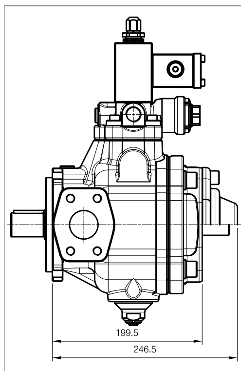
01 PHPK 2-(40-50-63) + Option "A" Single stage of pressure
