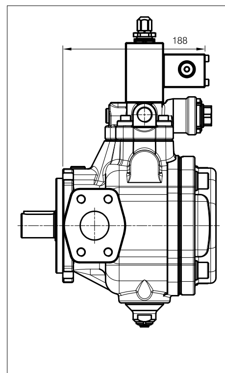
01 PHPK 2-(40-50-63) PCS003 pressure control
